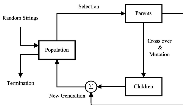
Fig. 6. A general scheme for Genetic Algorithm (Golpîra et al., 2011).
